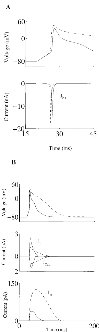
FIGURE 10 Simulated action potentials and the underlying ionic currents. (A) I_{\text{Na}} in the epicardial action potentials (solid line) and endocardial action potentials (dashed line). (B) I_{\text{CaL}} , I_t , and I_{\text{ss}} during the epicardial action potentials (solid line) and endocardial action potentials (dashed line).
