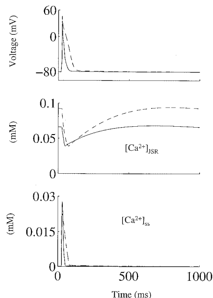
FIGURE 13 Simulated action potentials [Ca^{2+}]_{SR} and [Ca^{2+}]_{ss} in epicardial (solid line) and endocardial (dashed line) cells.
