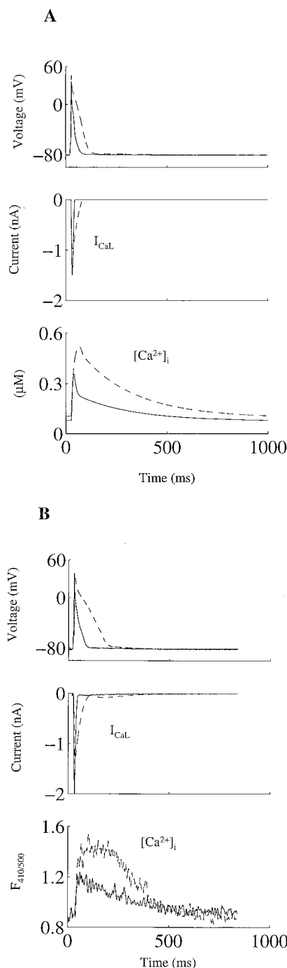
FIGURE 12 (A) Simulated action potentials and the underlying changes in I_{CaL} and [Ca^{2+}]_i for the epicardial (solid line) and endocardial (dashed line) myocytes. (B) Experimentally recorded action potentials and the underlying I_{CaL} and [Ca^{2+}]_i in epicardial myocytes under control conditions (solid line), and in the presence of 3 mM 4-AP (dashed line) (from Bouchard et al., 1995). Changes in the ratio of fluorescence intensity of indo 1 at 410 nm to that at 500 nm ( F_{410/500} ) were taken as a measure of changes in [Ca^{2+}]_i (Bouchard et al., 1995).
