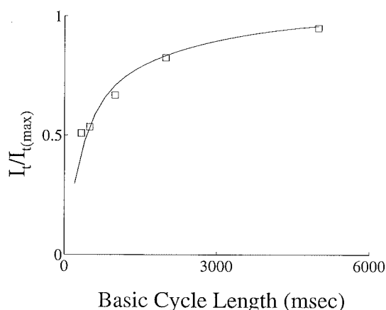
FIGURE 7 (A) Simulated current-voltage ( I - V ) curve for I_t in epicardial ( \circ , solid line) and endocardial ( \square , dashed line) myocytes, which were isolated from the adult rat left ventricle (cf. Shimoni et al., 1995). (B) Simulated recovery or reactivation characteristics for I_t as a function of the basic cycle length of stimulation in the endocardial cell. \square , Data obtained from the rate stimulation of I_t in rat endocardial myocytes. I_t was measured as the peak amplitude relative to zero (Shimoni et al., 1995).
