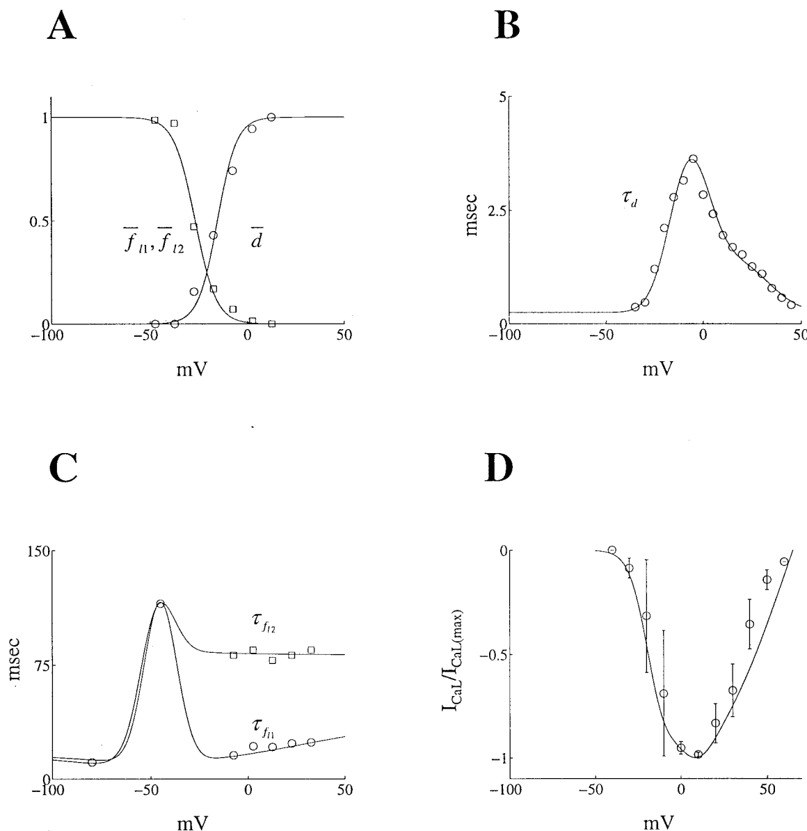
FIGURE 3 Parameters for the calcium current, I_{CaL} . (A) Steady-state activation ( \bar{d} ) and inactivation ( \bar{f}_{11} , \bar{f}_{12} ) ( \circ and \square represent data from Katsube et al., 1998). (B) Activation time constant ( \tau_d ) ( \circ represents data from Sun et al., 2000). (C) Inactivation time constants ( \tau_{f11} , \tau_{f12} ) ( \circ and \square represent data for fast and slow inactivation from Katsube et al., 1998, data at -50 mV and -80 mV being recovery from inactivation kinetics, from Meszaros et al., 1997 and Nawrath and Wegner, 1997, respectively). (D) Normalized simulated current-voltage ( I-V ) curve for I_{CaL} ( \circ represents normalized data from Richard et al., 1993).
