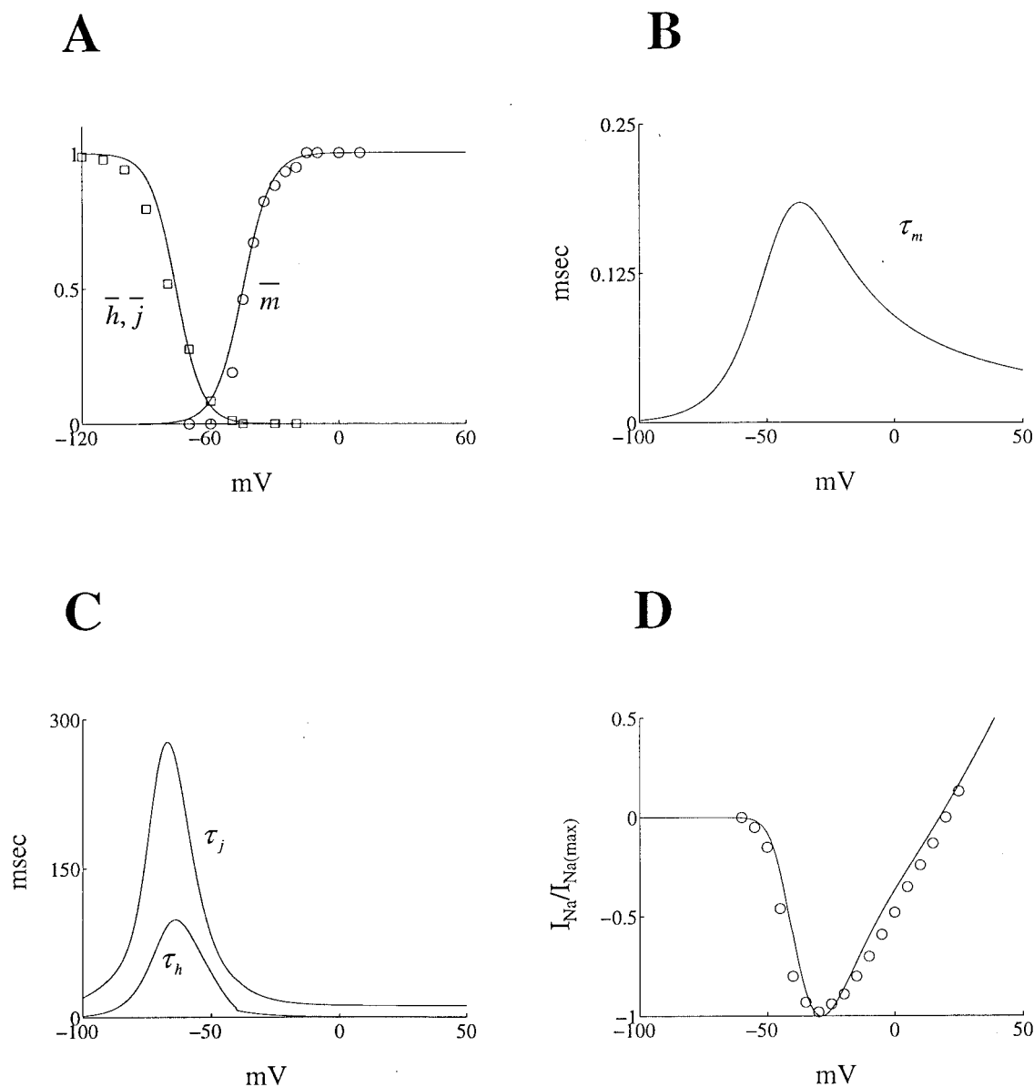
FIGURE 2 Parameters for the sodium current, I_{Na} . (A) Steady-state activation ( \bar{m} ) and inactivation ( \bar{h}, \bar{j} ) ( \circ and \square represent data from Lee et al., 1999). (B) Activation time constant ( \tau_m ) (scaled from Luo and Rudy, 1994). (C) Inactivation time constants ( \tau_h, \tau_j ) (scaled from Luo and Rudy, 1994). (D) Normalized simulated current-voltage ( I-V ) characteristics of I_{Na} ( \circ represents normalized data from Lee et al., 1999).
